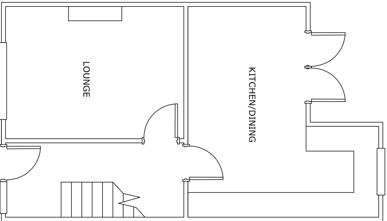
GROUND FLOOR PLAN (NOT TO SCALE)
